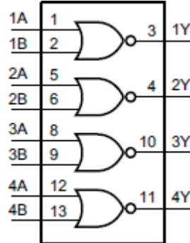
Figure 1. Functional diagram
