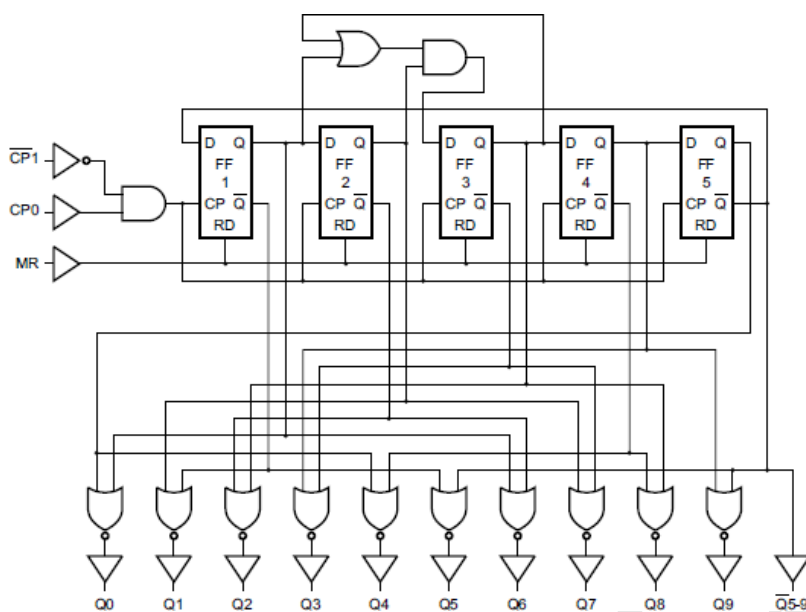
Figure 4. Logic diagram
