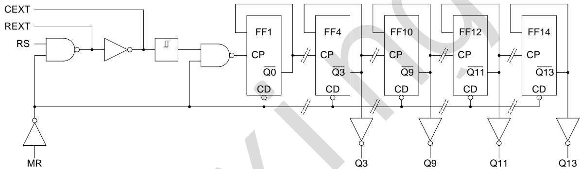
Figure 2. Logic diagram
