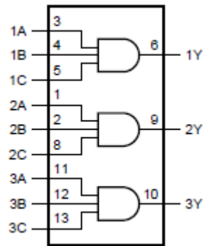
Figure 1. Functional diagram
