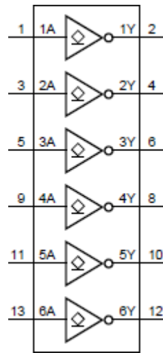
Figure 1. Logic symbol
