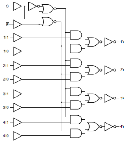
Figure 4. Logic diagram
