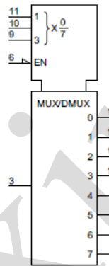
Figure 2. IEC logic symbol
