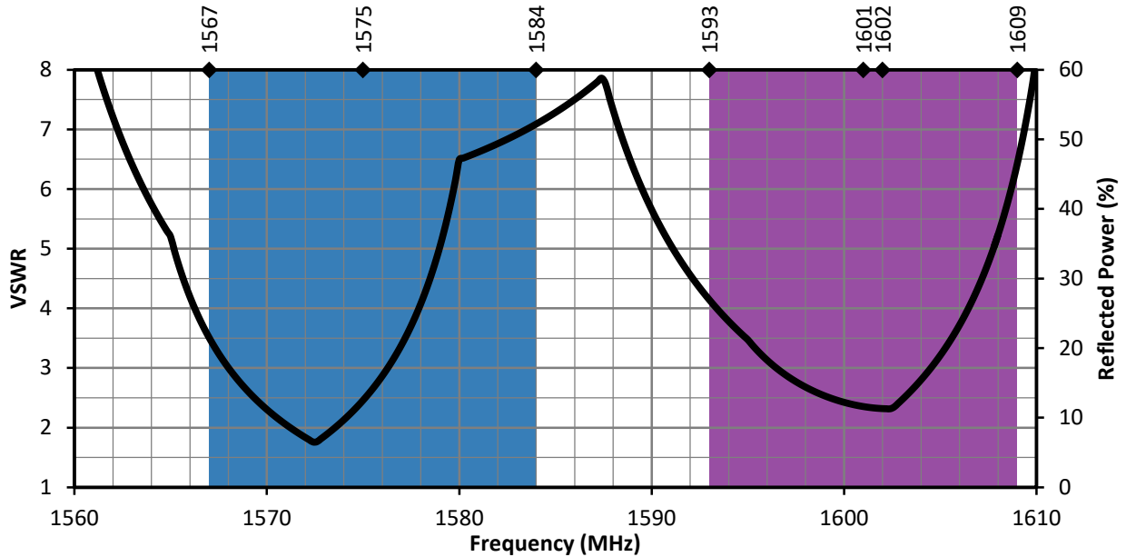
Figure 2. GNSSCP-SM12L1 VSWR
