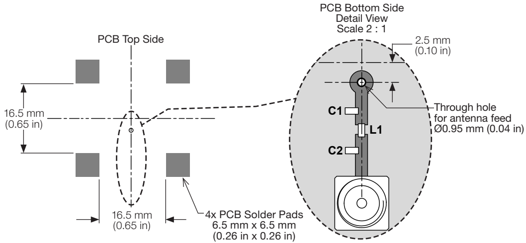
Figure 11. ANT-GNSSCP-TH25L1 Antenna Placement on PCB
