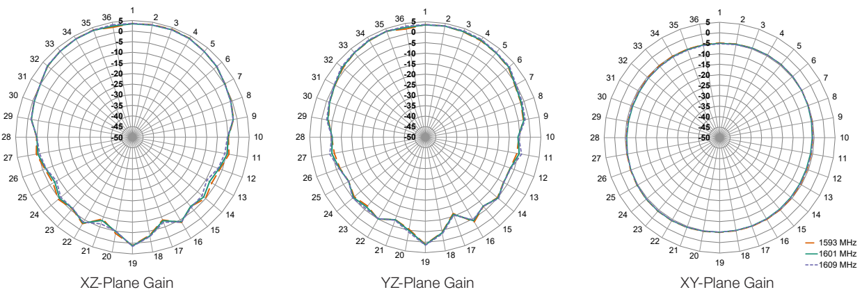
Figure 8. ANT-GNSSCP-TH25L1 Radiation Patterns
