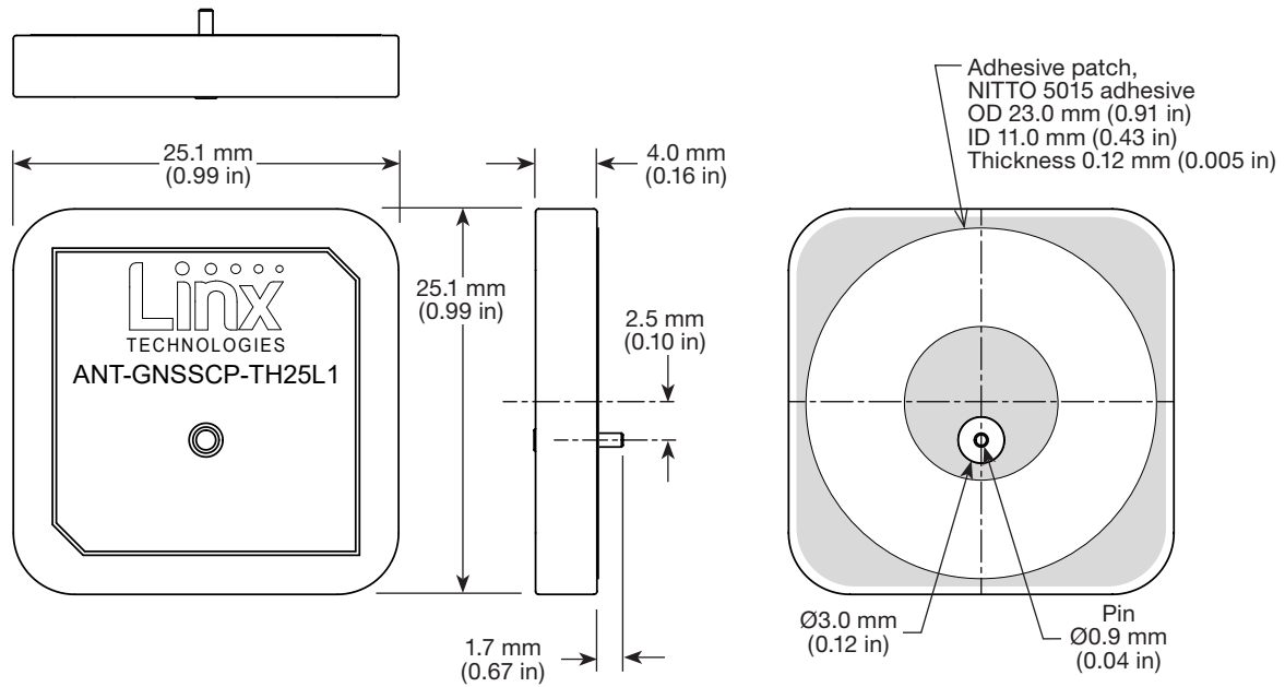
Figure 1. GNSSCP-TH25L1 Antenna Dimensions
