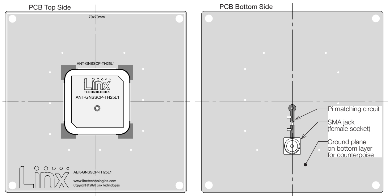
Figure 9. Recommended PCB Layout for the GNSSCP-TH25L1
