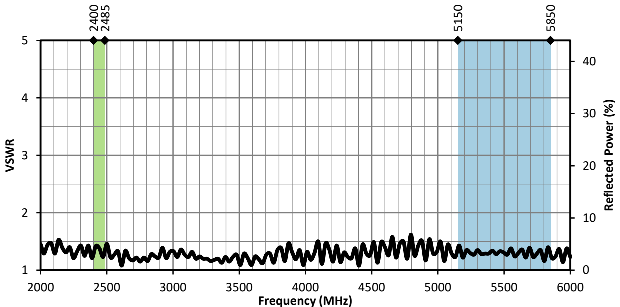
Figure 1. ANT-2/5-HDP-2000 Antenna VSWR, with Frequency Band Highlights
