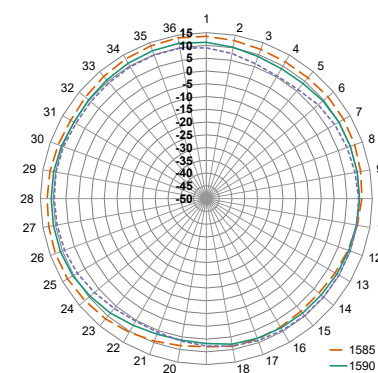
XY-Plane Gain
