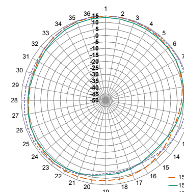
XY-Plane Gain
