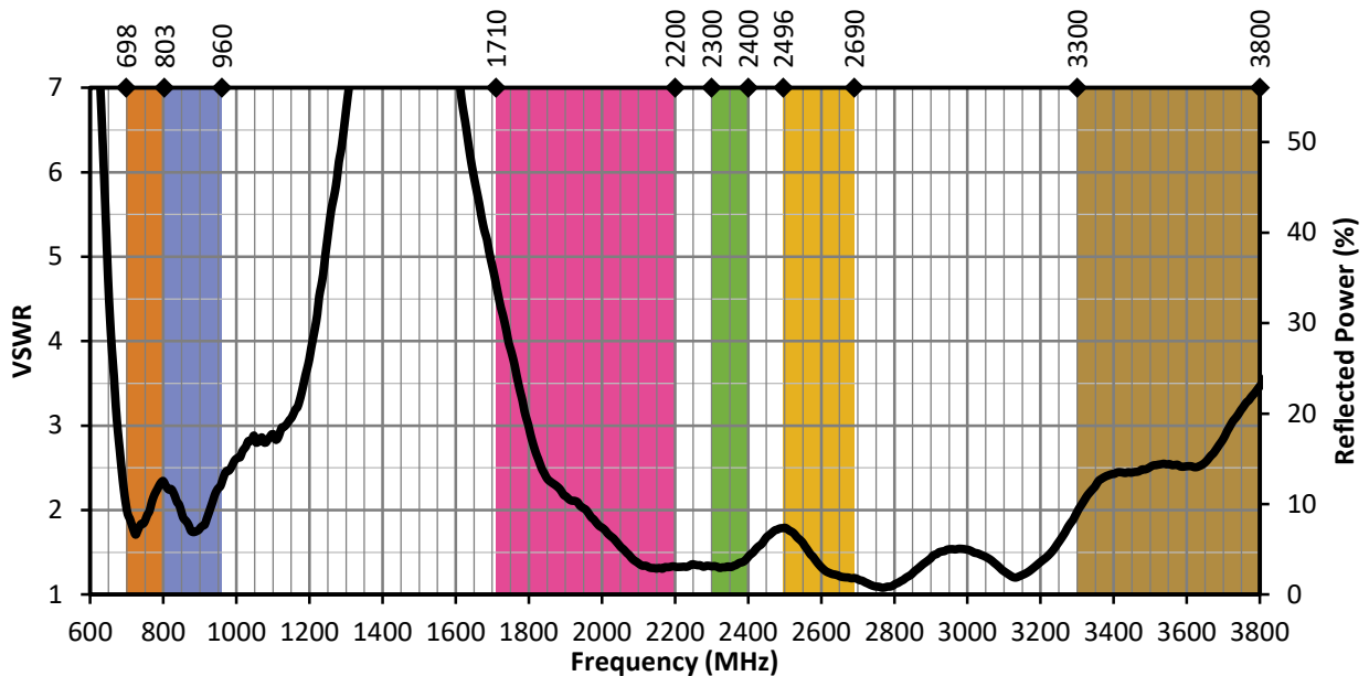
Figure 1. LPL Antenna VSWR with Frequency Band Highlights
