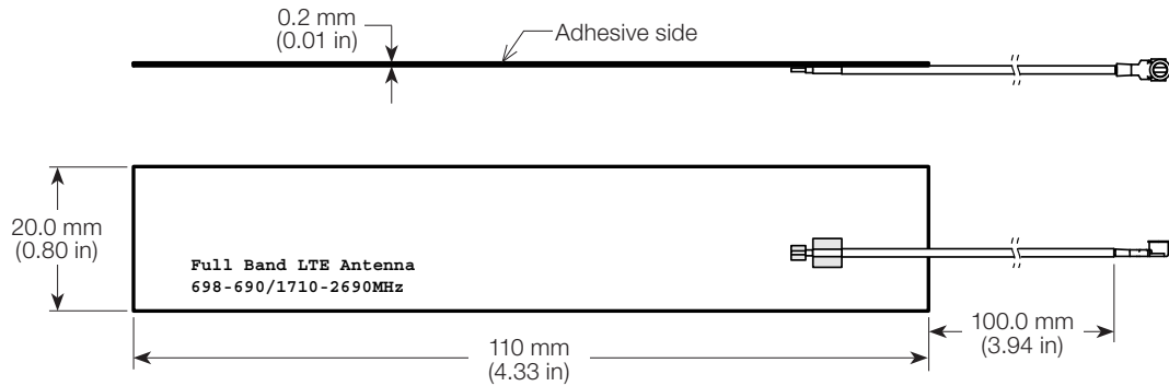
Figure 6. ANT-LPL-FPC-100 Dimensions
