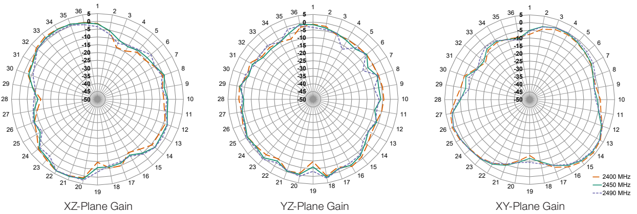
Figure 7. Radiation Patterns for ANT-LPL-FPC-100 Antenna
