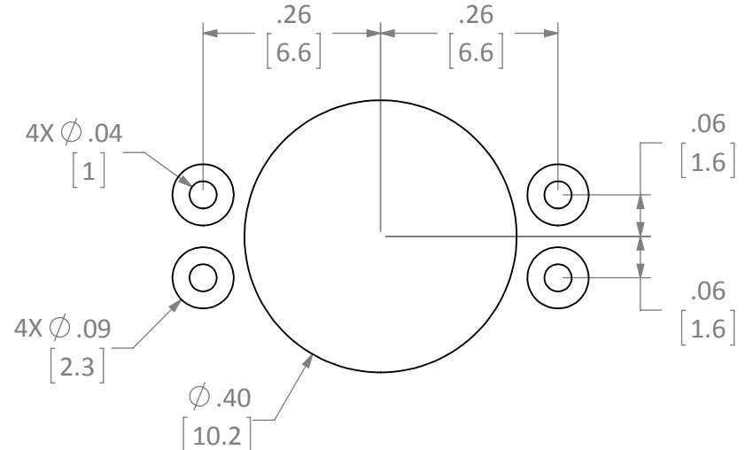
RECOMMENDED FOOTPRINT
