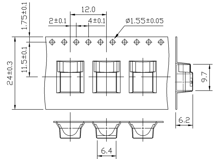
TAPE DIMENSIONS
