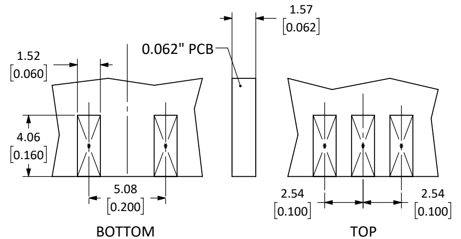
RECOMMENDED FOOTPRINT
