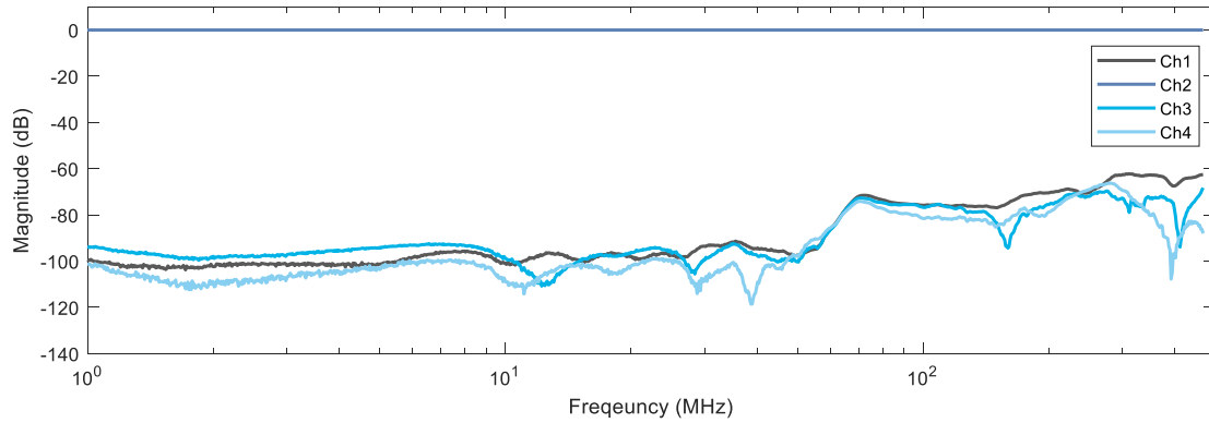
ADC 2 Crosstalk
