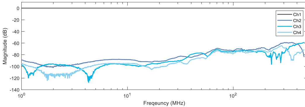
ADC 1 Crosstalk
