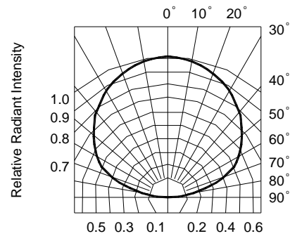
FIG.5 SENSITIVITY DIAGRAM
