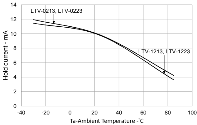
Fig 7. Hold current vs. Ambient Temperature
