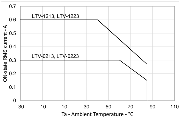
Fig 1. ON-state RMS current vs. Ambient Temperature
