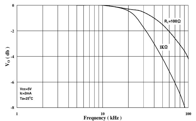
Figure 18. Frequency Response
