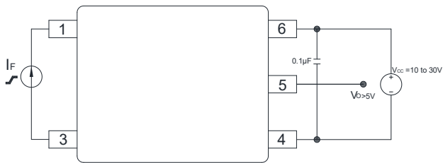
Figure 16 : I FLH Test Circuit
