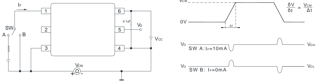
Figure 21 : CMR Test Circuit and Waveforms
