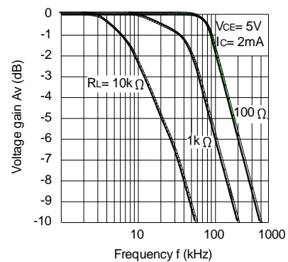
Fig.12 Frequency Response
