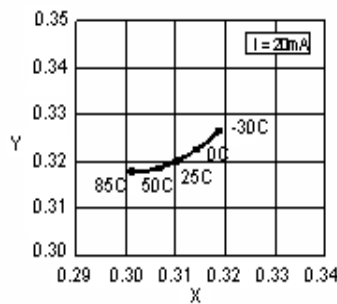
Fig.9 Ambient Temperature vs. Chromaticity Coordinate
