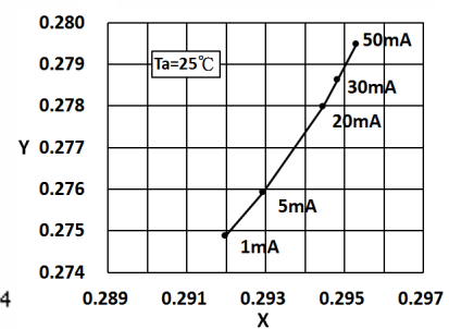
Fig.10 Forward Current vs. Chromaticity Coordinate
