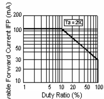
Fig.7 Duty Ratio vs. Allowable Forward Current
