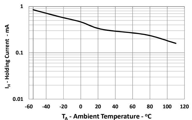
Fig.6 Holding Current vs. Ambient Temperature
