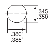
Mounting Hole
