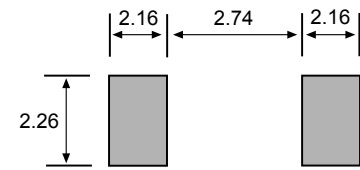
Solder Pads All dimensions in mm
