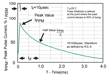
Fig. 3 Pulse Waveform
