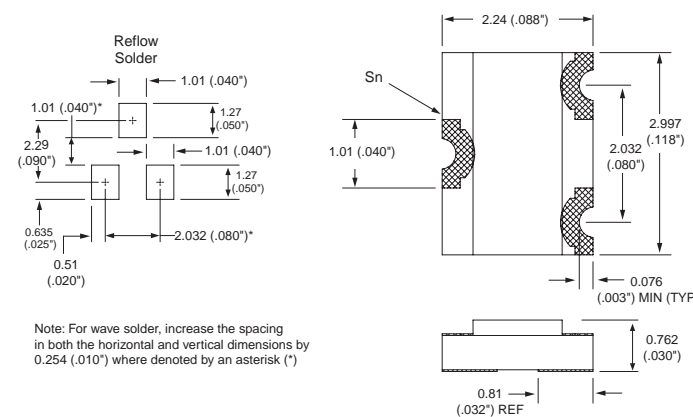
Reference Dimensions:
