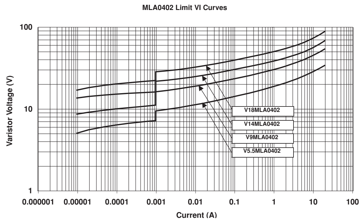
FIGURE 3. LIMIT V-I CHARACTERISTIC FOR V5.5MLA0402 TO V18MLA0402
