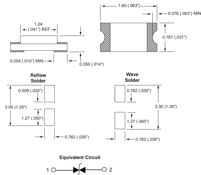
Reference Dimensions:
