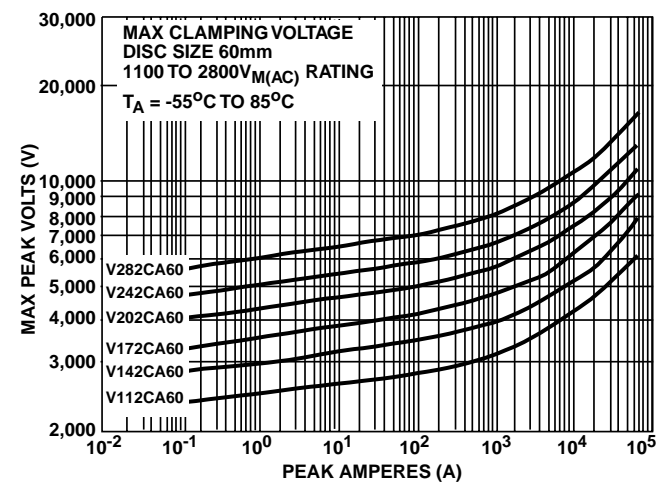
FIGURE 6. CLAMPING VOLTAGE FOR V112CA60 - V282CA60
