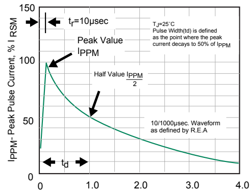
Fig. 3 Pulse Waveform
