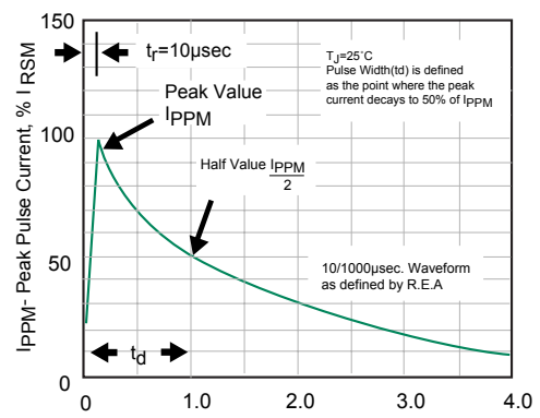
Fig. 3 Pulse Waveform
