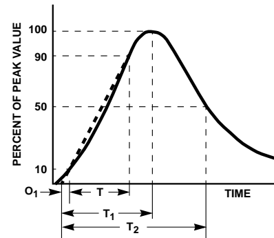
FIGURE 2. PEAK PULSE CURRENT TEST WAVEFORM
