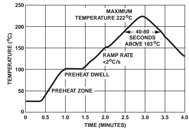
FIGURE 5. REFLOW SOLDER PROFILE
