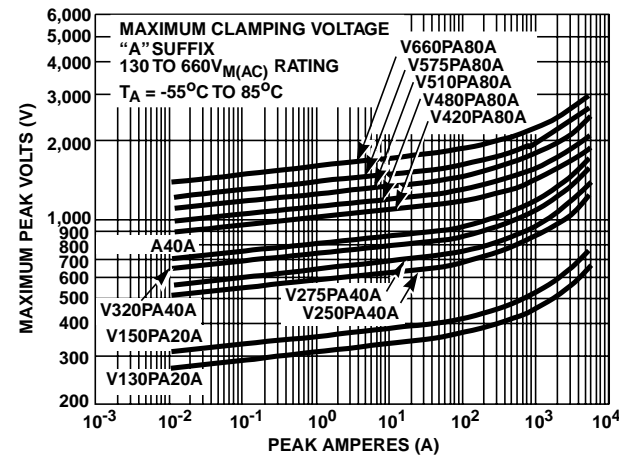
FIGURE 3. CLAMPING VOLTAGE FOR V130PA20A-V660PA100A
