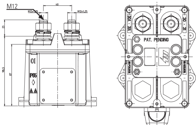
08097200 08097260 (with cover)
