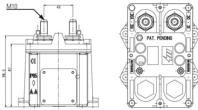
08097200 08097260 (with cover)
