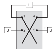
Forward-Reverse switch
