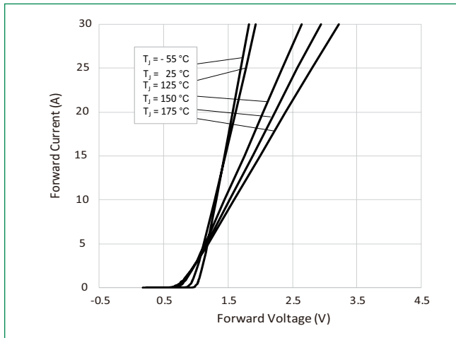
Figure 1: Typical Forward Characteristics (Per Leg)
