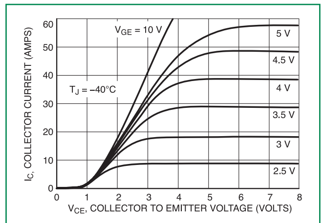
Figure 2. Output Characteristics
