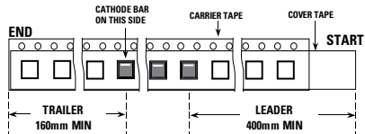
Leader and Trailer Dimension of the Ttape
