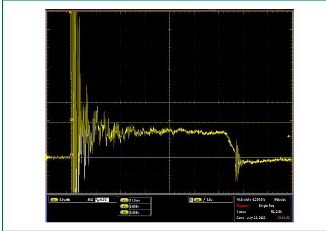
SC1115 IEC 61000 -4-2 +8 kV Contact ESD Clamping Voltage
