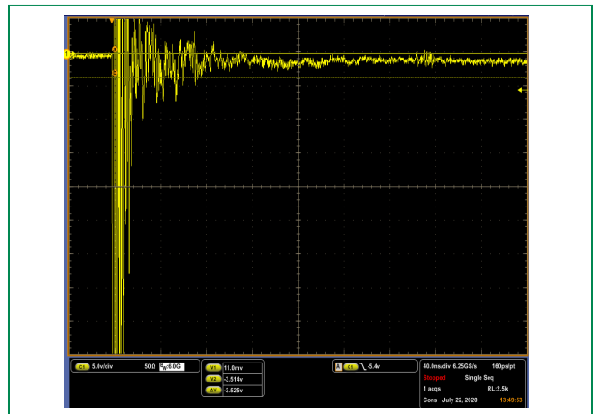
SC1122 IEC 61000 -4-2 -8 kV Contact ESD Clamping Voltage
