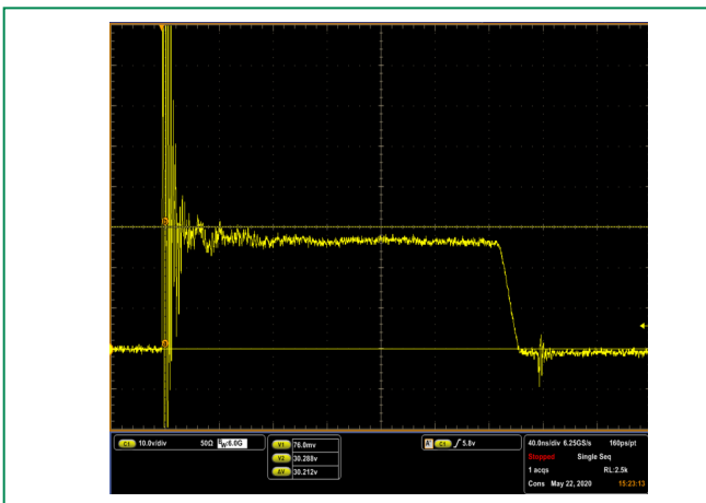
SC1122 IEC 61000 -4-2 +8 kV Contact ESD Clamping Voltage
