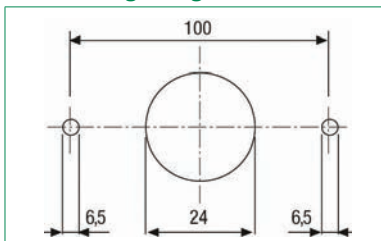
Mounting Diagram
