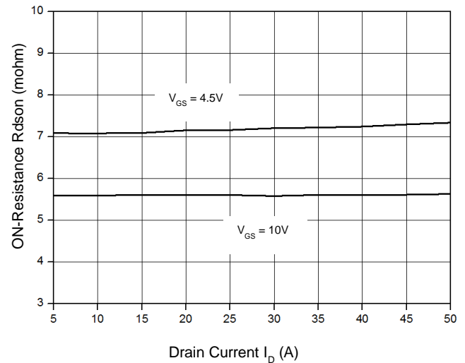
Figure 6. Rds(on)-Drain Current
