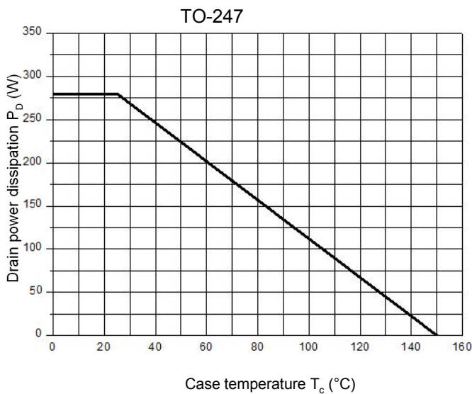
Figure 10.1 Power Dissipation vs. Temperature TO-247
