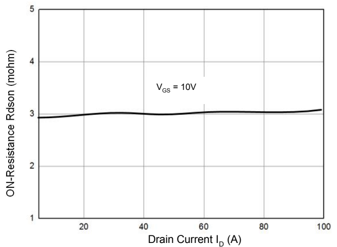
Figure 6. Rds(on)-Drain Current
