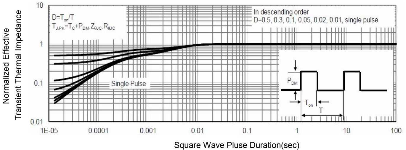
Figure 11. Normalized Maximum Transient Thermal Impedance (R thJC )
