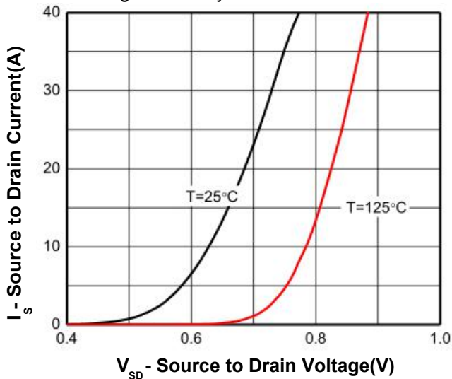
Figure 5. Body-Diode Characteristics
