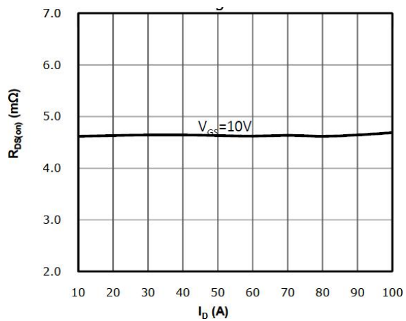
Figure 6. Rdson-Drain Current
