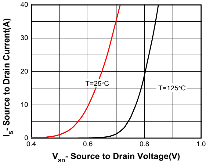
Figure 5. Body-Diode Characteristics
