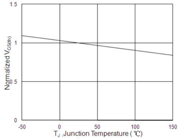
Figure 8. V GS(th) -Junction Temperature
