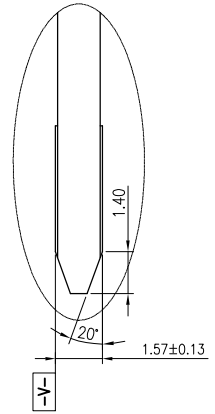
DETAIL "A" SCALE 4:1
