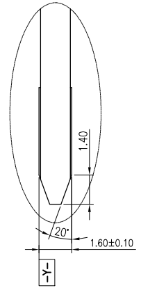
DETAIL "B" SCALE 4:1
