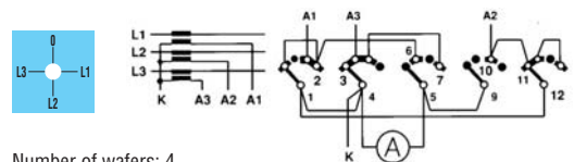
98 - L1-L2-L3 current changeover / double throw switch
