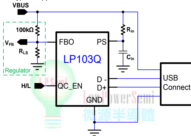
Figure 1B. Typical Application Circuit of LP103Q with SOT23-6 Package Type.
