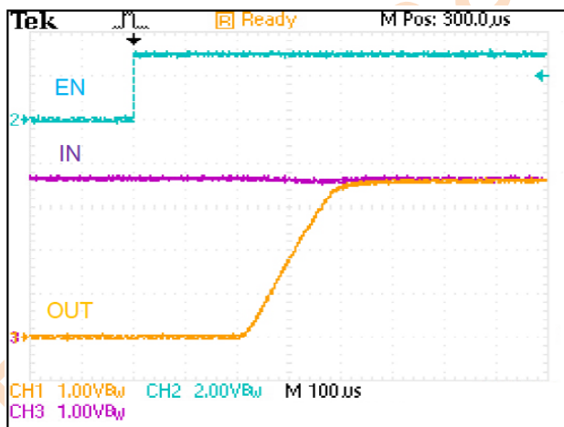
Figure 2. Turn on with EN pin ( C_{IN}=1\mu F , C_{OUT}=1\mu F , V_{IN}=3.6V , R_{LOAD}=25\Omega )
