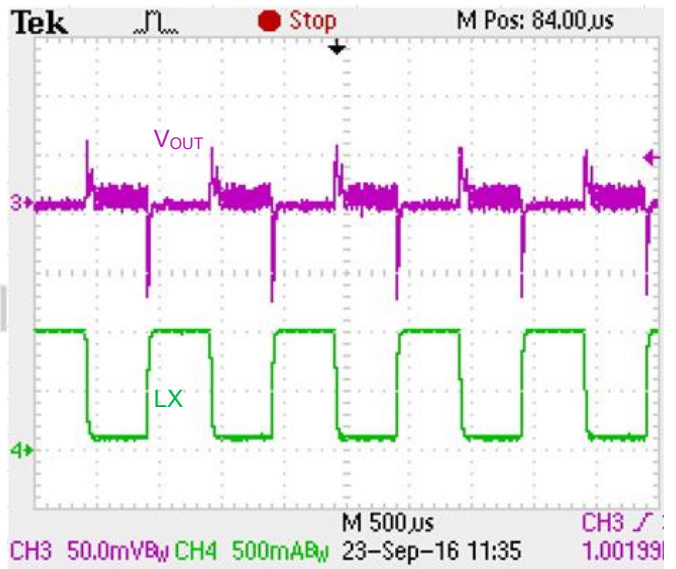
Output waveform @V OUT =3.3V, I o =100mA to 1A
