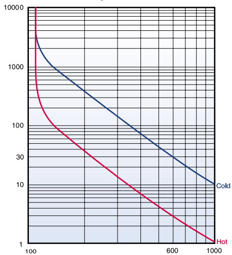
Trip class 30
