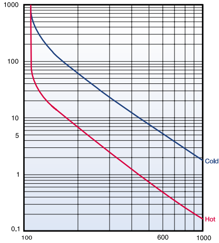
Trip class 5
