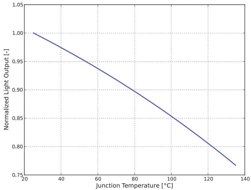
Figure 2. Typical normalized light output vs. junction temperature for LUXEON 2835 with FreshFocus Technology at 120mA.
