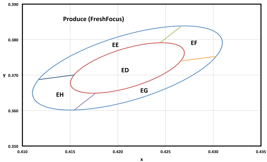
Figure 8a. 1/5 th color bin structure for LUXEON 2835 with FreshFocus Technology for Produce, 120mA, T_j=25^\circ\text{C} .
