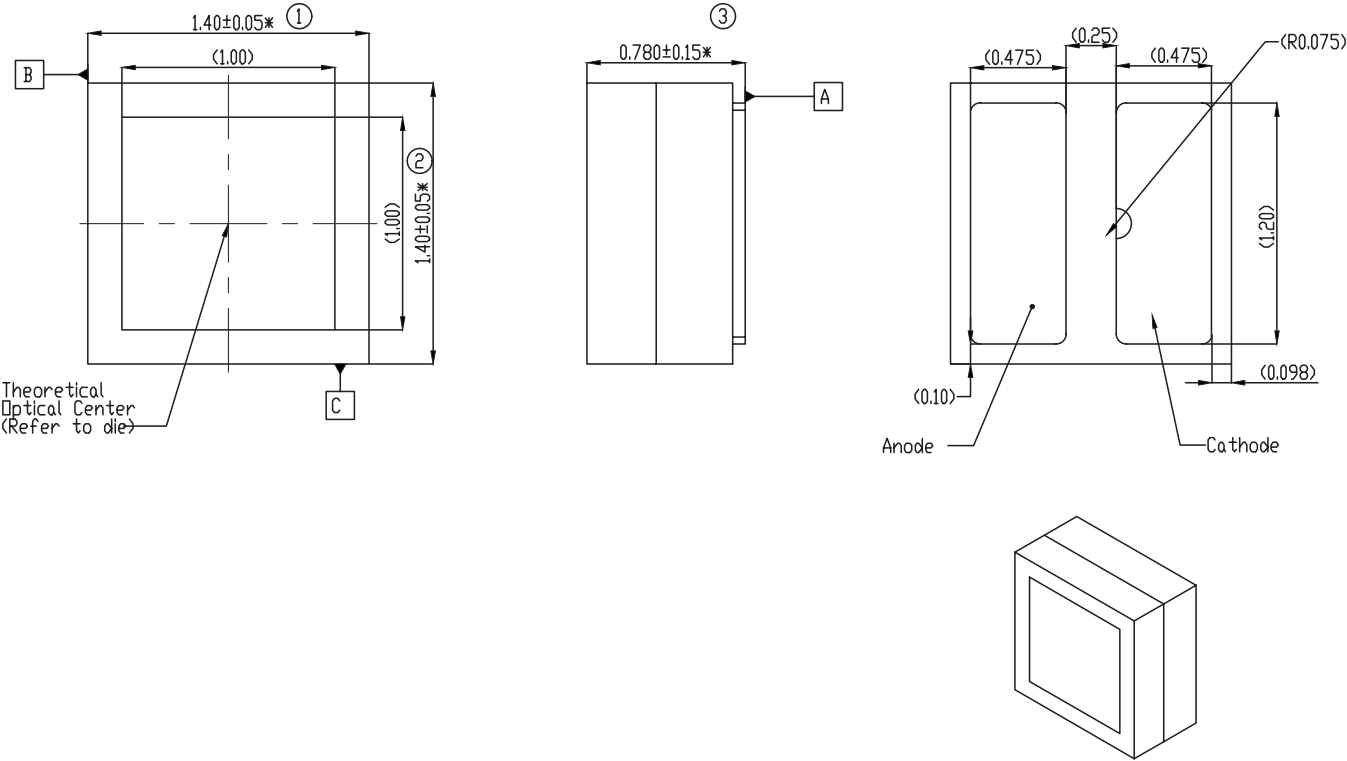
Figure 9a. Mechanical dimensions for LUXEON Rubix Green, Blue, Royal Blue and White Colors.
