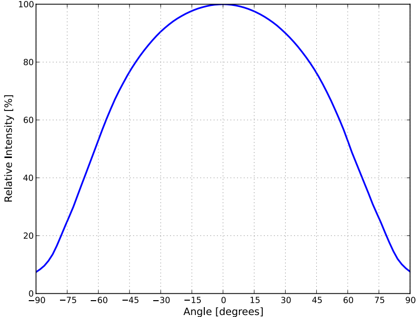
Figure 6. Typical radiation pattern for LUXEON V at 1400mA, T j =85°C.
