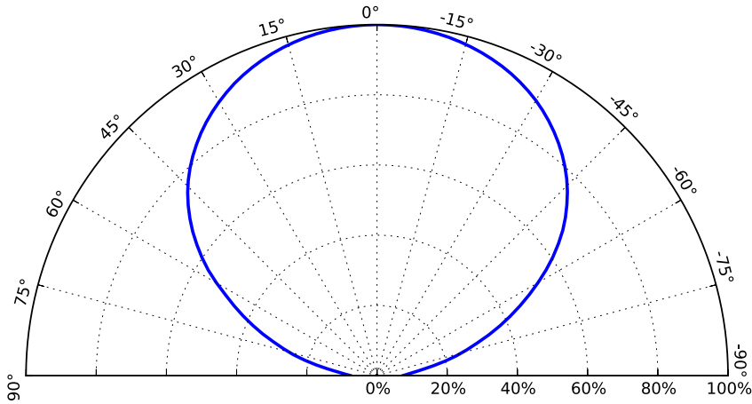
Figure 7. Typical polar radiation pattern for LUXEON V at 1400mA, T j =85°C.
