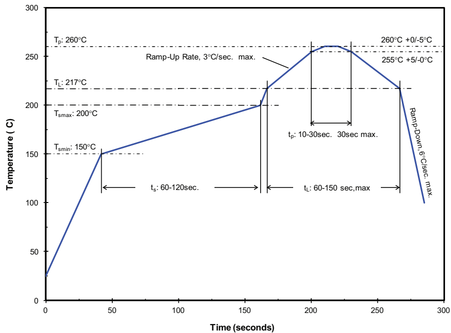
Figure 1. Temperature profile for Table 7.
